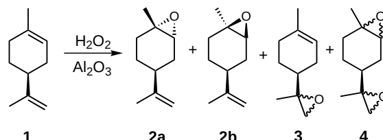
Figure 1. Epoxidation of ( S )-limonene.
